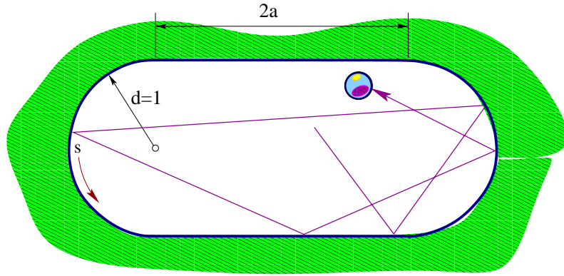
Figure 9.1: The stadium billiard [9.9, 9.10] is a 2-dimensional domain bounded by two semi-circles of radius d = 1 connected by two straight walls of length 2a . At the points where the straight walls meet the semi-circles, the curvature of the border changes discontinuously; these are the only singular points of the flow. The length a is the only parameter.
