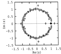
Figure 15.3: The 90 zeros of the topological zeta function for the quadratic map for A = 3.8 approximated by the nearest topological zeta function with a stable cycle of length 90. (from K.T. Hansen [12.20])
