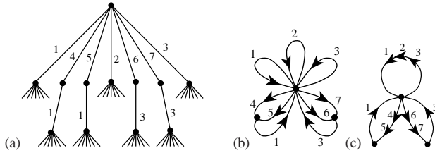
Figure T.2: (a) The sawtooth map (T.1) partition tree for figure T.1 (a); while intervals M_1, M_2, M_3 map onto the whole unit interval, f(M_1) = f(M_2) = f(M_3) = M_1 , intervals M_4, M_5 map onto M_1 only, f(M_4) = f(M_5) = M_1 , and similarly for intervals M_6, M_7 . An initial point starting out in the interval M_1, M_2 or M_3 can land anywhere on the unit interval, so the subtrees originating from the corresponding nodes on the partition three are similar to the whole tree and can be identified (as, for example, in figure 10.13), yielding (b) the Markov graph for the Markov partition of figure T.1 (a). (c) the Markov graph in the compact notation of (24.26).
