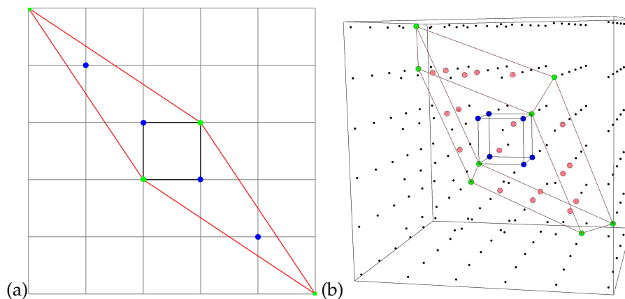
Figure 15.21: (a) A 2-dimensional torus (with black border) stretched by \mathcal{J} . The blue dots are internal integer points in the fundamental parallelepiped (with red border). The green dots are on the vertices of the fundamental parallelepiped. (b) A 3-dimensional torus (with black border) stretched by \mathcal{J} . The blue dots are internal integer points in the stretched fundamental parallelepiped (with red border). The green dots are on the vertices of the fundamental parallelepiped. The pink dots are on the surface of the fundamental parallelepiped.
