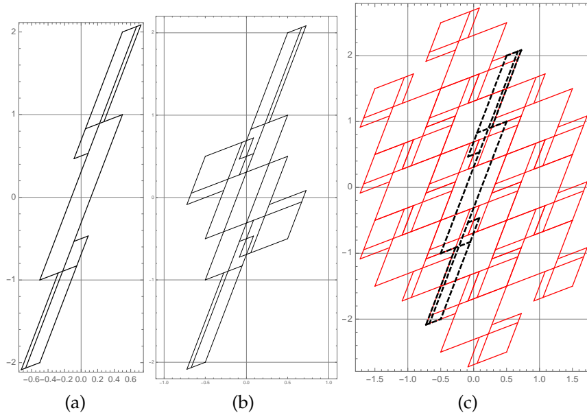
Figure 20.16: (a) The forward image of the 7-rectangle partition figure 20.15 (b). (b) The stretched partition overlaid over the original partition. (c) The stretched partition overlaid over the tiled lattice. The x and y axes are not plotted to the same scale.
