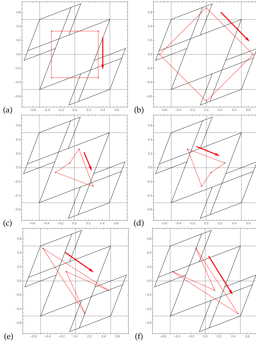
Figure 20.18: All 4-cycles from (20.22): (a) \Phi_{1111} (b) \Phi_{0202} , (c) \Phi_{0011} , (d) \Phi_{0011} , (e) \Phi_{1122} , (f) \Phi_{2211} , (g) to (j) continued in figure 20.20.
