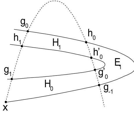
Figure 9.1: A sketch of a partial homoclinic tangle which forms a complete horseshoe structure. The unstable (stable) manifold of x is the solid (dashed) curve. There are two primary homoclinic orbits \{h_0\} and \{g_0\} . \mathcal{R} is the closed region bounded by loop \mathcal{L}_{USUS[x, g_{-1}, h_0, g_0]} . (From ref. [39])
