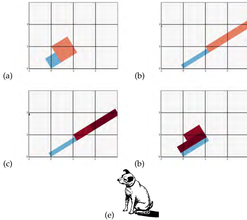
Figure 20.1: Figure 1.1 recomputed with my python code. (a) Two-squares Adler-Weiss generating partition for the canonical Thom-Arnol'd cat map (1.1), with borders given by stable-unstable manifolds of the unfolded cat map lattice points near to the origin. (b) The first iterate of the partition. (c) The first iterate of the partition intersections, (d) The iterate pulled back into the generating partition, and (e) the corresponding 5-letter transition graph. In (b) and (c) we still have to relabel Crutchfield's arbitrary partition labels with our shift code. This is a "linear code," in the sense that for each square one can count how many side-lengths are needed to pull the overhanging part of (c) back into the two defining squares.
