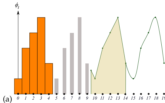
Figure 20.64: For a time-reversal invariant system, a period n lattice state \Phi , plotted here as the field values \phi_t , each bar centred at lattice site t , has one of the 4 possible symmetries, illustrated by: (a) A period-5 lattice state \Phi invariant under the translation group H(5) , with no time reversal symmetry.
