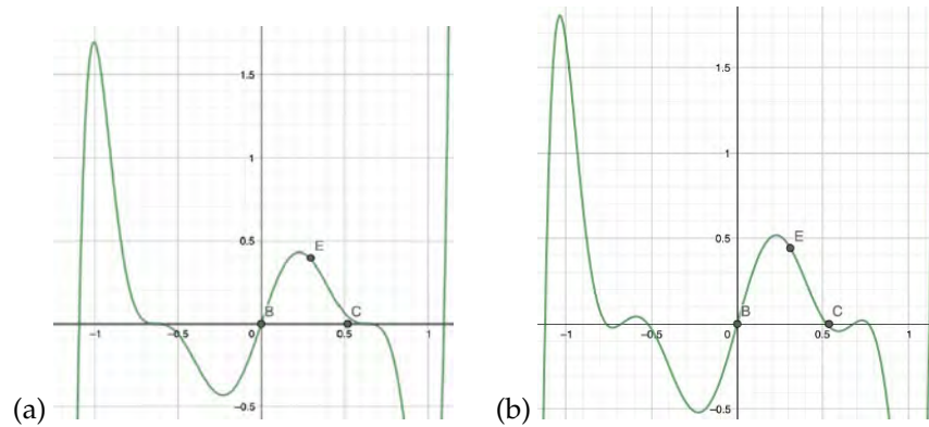
Figure 19.5: \phi^4 theory (3.36) unwritten function g(\phi) = \phi(A\phi^8 + B\phi^6 + C\phi^4 + D\phi^2 + E) , whose zeros have something to do with period-2 lattice states. (a) s = 4 is the bifurcation value, corresponding to \mu^2 = s - 2 = 0 in (3.36). For higher s values all nine roots are real, for example for (b) s = 4.4 .
