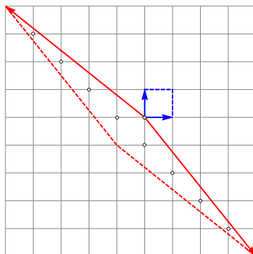
Figure 15.23: The fundamental parallelepiped of a [2 \times 1]_1 invariant 2-torus with s = 5/2 . Admissible field values lie within the unit square with blue boundaries. This unit square is stretched by the orbit Jacobian matrix \mathcal{J} into the fundamental parallelepiped with red boundaries. Integer points in the fundamental parallelepiped are marked by the circles. There are 9 integer points in the fundamental parallelepiped, in agreement with the counting formula.
