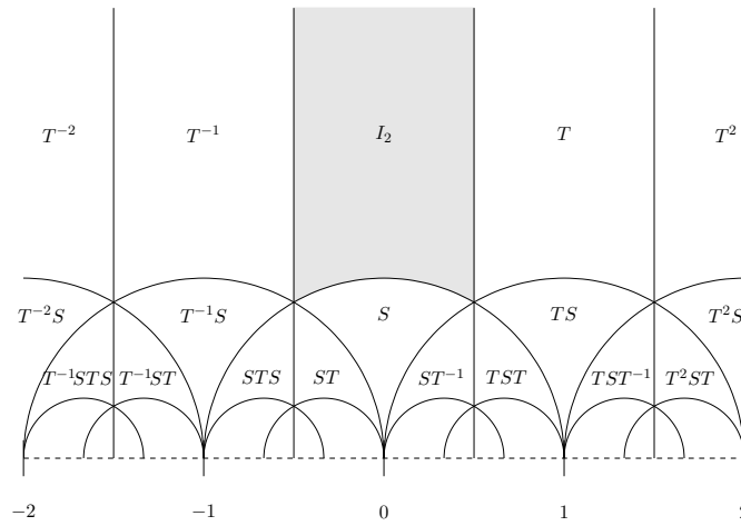
Figure 13.2: Action of SL_2(\mathbb{Z}) on the complex upper half-plane by linear fractional transformations T and S . Taken from Keith Conrad.
