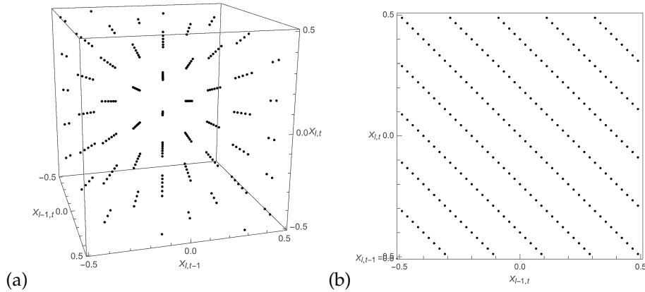
Figure 20.29: (a) All of the points in the periodic [2 \times 2] blocks. The coordinates of each points are \phi_{l-1,t} , \phi_{l,t-1} and \phi_{lt} . (b) The front view of (a). Clearly these points are arranged in lines.
