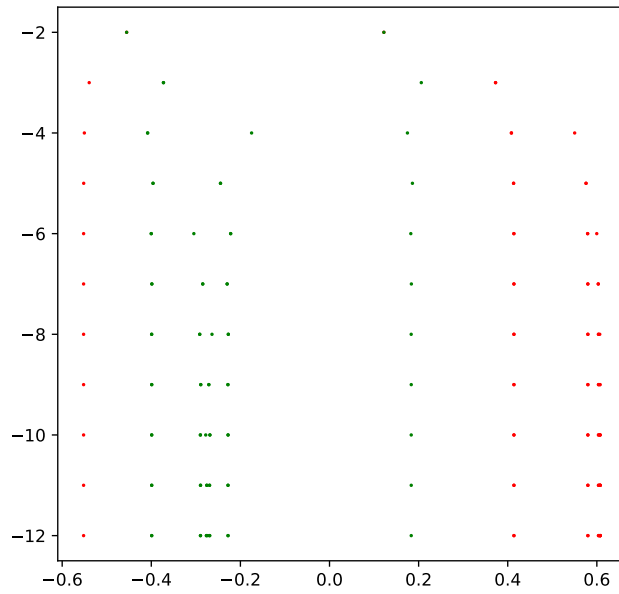
Figure 16.8: Plotting 1000... (Red one negative lattice state) and 01111... (Green one positive lattice state), by orbit length
