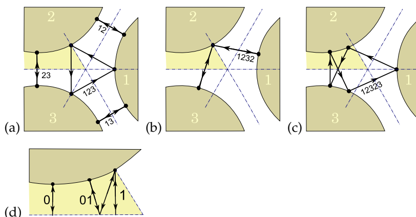
Figure 5.9: The 3-disk pinball orbits: (a) \overline{12} , \overline{13} , \overline{23} , \overline{123} ; the clockwise \overline{132} not drawn. (b) Orbit \overline{1232} ; the symmetry related \overline{1213} and \overline{1323} not drawn. (c) Orbit \overline{12323} ; orbits \overline{12123} , \overline{12132} , \overline{12313} , \overline{13131} and \overline{13232} not drawn. (d) The fundamental domain, i.e., the light-shaded 1/6th wedge in (a), consisting of a section of a disk, two segments of symmetry axes acting as straight mirror walls, and the escape gap to the left. The above 14 full-space orbits restricted to the fundamental domain and recoded in binary reduce to the two fixed points \overline{0} , \overline{1} , period-2 orbit \overline{10} , and period-5 orbit \overline{00111} (not drawn).
