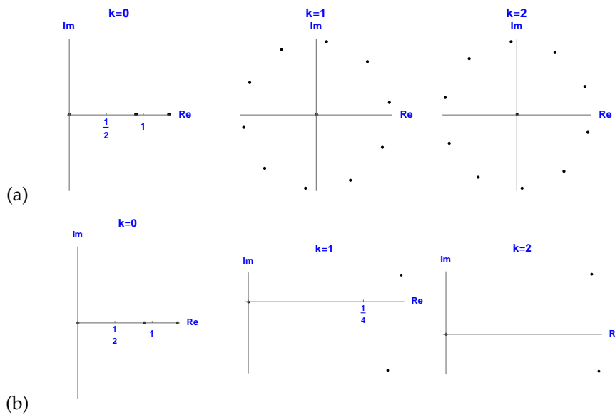
Figure 20.55: (a) The \tilde{N}_5 = 11 period n = 5 reciprocal lattice states of the 1/2 time step lattice (temporal golden cat) of the s = 3 temporal cat, obtained by discrete C_5 irreps diagonalization. (b) The C_5 symmetry-reduced fundamental domain contains \tilde{M}_5 = 2 prime reciprocal lattice states whose phases lie in [-2\pi/10, 2\pi/10) , one prime reciprocal lattice state for each C_5 group orbit. The constant lattice state \{0, 0, 0, 0, 0\} lives in the intersection of the fundamental domain and its images.
