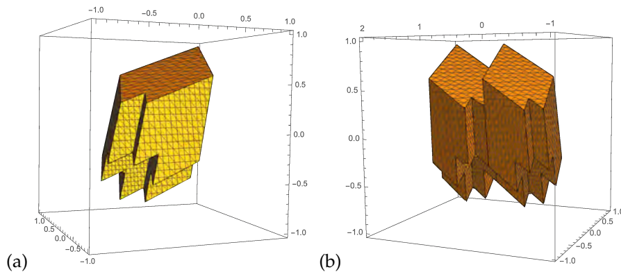
Figure 20.36: (a) A tiling region in three-dimensions. (b) The tiling region and one nearest neighboring region. You can see the boundaries exactly matched.
