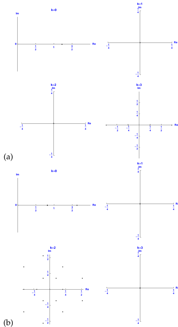
Figure 20.58: The period-6 reciprocal lattice states of the temporal cat with s = 3 , obtained by discrete C_6 irreps diagonalization. (a) The reciprocal lattice states in the subspace of C_2 , whose components are non-zero only in the k = 0 and k = 3 subspace. These lattice states are repeats of period-2 lattice states. (b) The reciprocal lattice states in the subspace of C_3 , whose components are non-zero only in the k = 0, k = 2 and k = 4 subspace. These lattice states are repeats of period-3 lattice states.
