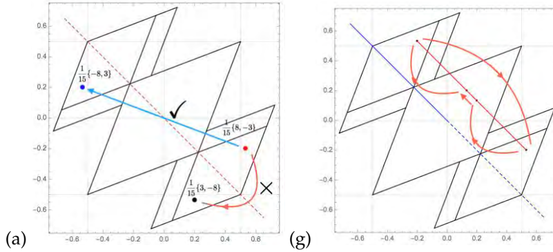
Figure 20.27: (a) The space inversion operation. Point (-8/15, 3/15) happens to be a periodic point of period 4, cycle \overline{1012} \rightarrow \overline{CAAB} , see (20.18) (g,h). Actually, any fractional coordinate belongs to a periodic orbit. The orange line is here just to confuse you; under inversion (3/15, -8/15) maps into (-3/15, 8/15) (not drawn). (g) The two corresponding 4-cycles reduced to a single 4-cycle in the space inversion fundamental domain, \overline{1012} and \overline{1012} \rightarrow \overline{CAAB} .
