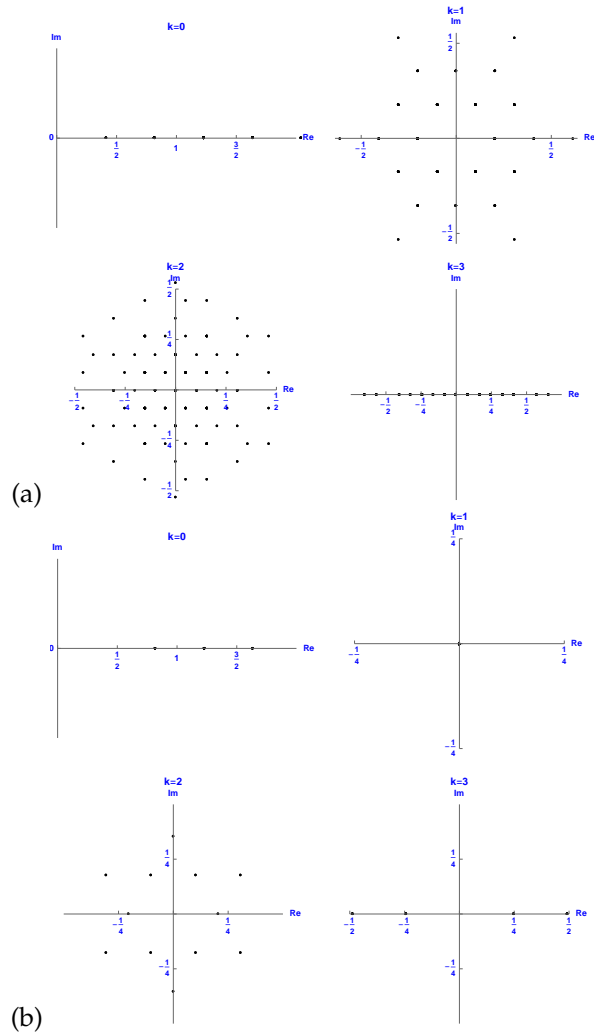
Figure 20.59: The period-6 reciprocal lattice states of the temporal cat with s = 3 , obtained by discrete C_6 irreps diagonalization. (a) The reciprocal lattice states that are not in the subspace of C_2 or C_3 , which have non-zero component in the k = 1 subspace. (b) The reciprocal lattice states that are not in the subspace of C_2 or C_3 , which have zero component in the k = 1 subspace and non-zero components in the k = 2 and k = 3 subspaces.
