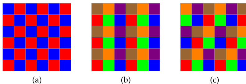
Figure 11.2: Examples of [\ell \times \ell]_S periodic blocks together with their spatiotemporal Bravais lattice tilings (??). (a) [2 \times 1]_1 , basis vectors \mathbf{a}_1 = \{2, 0\} and \mathbf{a}_2 = \{1, 1\} ; (b) [3 \times 2]_0 , basis vectors \mathbf{a}_1 = \{3, 0\} and \mathbf{a}_2 = \{0, 2\} ; (c) [3 \times 2]_1 , basis vectors \mathbf{a}_1 = \{3, 0\} and \mathbf{a}_2 = \{1, 2\} ;
