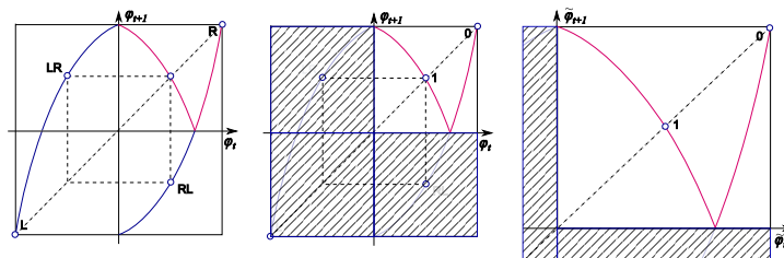
Figure 5.8: The ‘bent Bernoulli’ map of figure 5.7 with the D_1 symmetry f(-\phi) = -f(\phi) , restricted to the fundamental domain. f(\phi) is indicated by a blue line, and fundamental domain map \tilde{f}(\tilde{\phi}) by the purple line. The asymmetric fixed point pair \{\bar{L}, \bar{R}\} is reduced to the fixed point \bar{0} , and the full state space symmetric 2-cycle \bar{LR} is reduced to the fixed point \bar{1} . (work through example 5.11)
