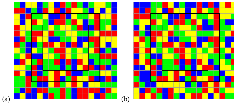
Figure 15.6: Figure nixed by Boris 2019-08-21, replaced by digits figure ?? Symbolic representation (colored tiles) of two [L \times T] = [18 \times 18] invariant 2-torus solutions of (??), s = 7 , that shadow each other within the shared block M_{\mathcal{R}} = M_{\mathcal{R}_0} \cup M_{\mathcal{R}_1} (blue). The symbols within \mathcal{R} , drawn randomly from the interior alphabet \mathcal{A}_0 , are the same for both solutions; the symbols outside \mathcal{R} , also drawn randomly from \mathcal{A}_0 , differ. The shared block \mathcal{R} = \mathcal{R}_0 \cup \mathcal{R}_1 is split into the interior region \mathcal{R}_0 (bold blue) and the border strip \mathcal{R}_1 (blue).
