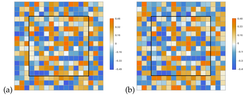
Figure 15.12: (a) and (b) are two invariant 2-tori whose symbol arrays are given by the [18 \times 18] blocks of symbols of figure 15.11.
