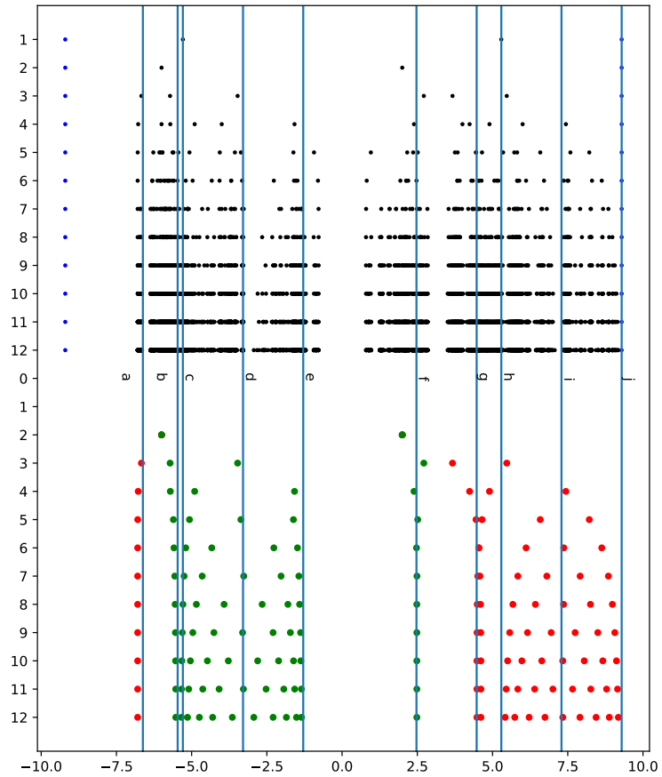
Figure 16.4: a = 6 temporal Hénon (2.3) with Smale horseshoe indicated in figure 4.2. (top frame) orbit Jacobian matrix eigenvalues for all prime orbits of periods n = 1 to 12, plotted on top of each other, with \bullet Gershgorin bounds. (bottom frame) The eigenvalues of (red) 10^{n-1} and (green) 01^{n-1} . The vertical blue lines indicate various \lambda values. The fixed points (2.4) field values (\phi_0, \phi_1) appear to be the centers of the Christmas trees at d = 2a\phi_1 and i = 2a\phi_0 , bracketed by c = 2a\phi_1 - 2 = the minimum, and e = 2a\phi_1 + 2 = maximum Gershgorin bound for \phi_1 ; and h = 2a\phi_0 - 2 = the minimum, and j = 2a\phi_0 + 2 = the maximum Gershgorin bound of \phi_0 . Eigenvalue series are also converging to values that presumably have nothing to do with the 10^{n-1} and 01^{n-1} orbits. Period-2 orbit (2.5) field values are (\phi_{10}, \phi_{01}) : b = 2a\phi_{10} seems close to a series, but not quite. I know numerically calculated period-3 orbit field values: f = \sqrt{6} = 2 \times the center value of \overline{101} seems pretty good (at least until I start plotting the differences), g = 4.47213 \dots which is twice either positive value in \overline{010} is off the mark, and so is a = -6.6204 \dots = , which 2 \times the center value of \overline{11011} .
