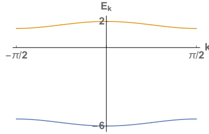
Figure 20.70: The eigenvalue E_k of the period-2 a = 6 Hénon's orbit Jacobian matrix on the infinite lattice as a function of the wave vector k .
