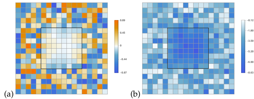
Figure 15.16: (a) The pointwise distance between the two invariant 2-tori of figure 15.15. (b) The logarithm of the absolute value of the distance between the two invariant 2-tori indicate exponential shadowing close to the center of the shared M_{\mathcal{R}} .
