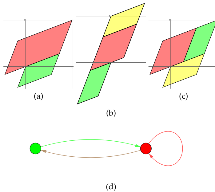
Figure 20.57: (a) An Adler-Weiss generating partition of the unit torus for the golden cat map (1/2 time step map) (6.115), (20.72), the time-reversal reduction of the s = 3 or \mu = 1 Percival-Vivaldi cat map (1.5) and figure 1.9, with rectangle \mathcal{M}_A (red) and \mathcal{M}_B (green) borders given by the stable and unstable manifolds, i.e., along the two eigenvectors corresponding to the eigenvalues of the matrix \tilde{C} in (20.72). (b) Mapped one half time-step forward in time, the rectangles are stretched along the unstable direction and shrunk along the stable direction. The eigenvectors are the same as for the Percival-Vivaldi cat map, but eigenvalue \tilde{\Lambda} (6.116) is a square root of the Percival-Vivaldi cat map eigenvalue (1.6), \Lambda = \tilde{\Lambda}^2 , hence less stretching. (c) As always, the sub-rectangles translated back into the initial partition yield a generating partition, with the finite grammar given by the transition graph (d) of figure 5.2. The nodes refer to the green and red rectangles, and the three links correspond to the three sub-rectangles induced by one forward half time-step.
