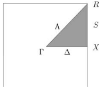
Figure 5.3: The shaded (or yellow) area indicates a fundamental domain , i.e., the smallest part of the pattern whose repeats tile the entire plane. For the most symmetric 2D square lattice, with point group p4mm , the fundamental domain is indicated by the shaded triangle \Gamma\Delta RSX\Delta\Gamma which constitutes 1/8 of the Brillouin zone, and contains the basic wave vectors and the high symmetry points (Fig. 10.2 of Dresselhaus et al. [32]).
