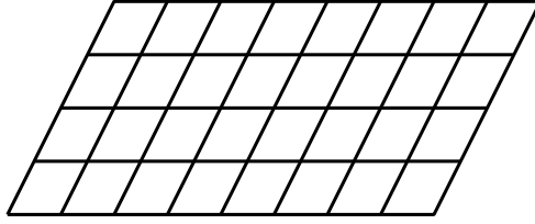
Figure 13.1: \ell \times \ell square lattice with tilt parameter c . Here, \ell = 8 , \ell = 4 and c = 1/4 , so S = \ell/4 . The i -th site of the first row is identical with the \text{mod}(i + c\ell, \ell) -th site in the last row. The left-most site and the right-most site on the same horizontal line are identical.
