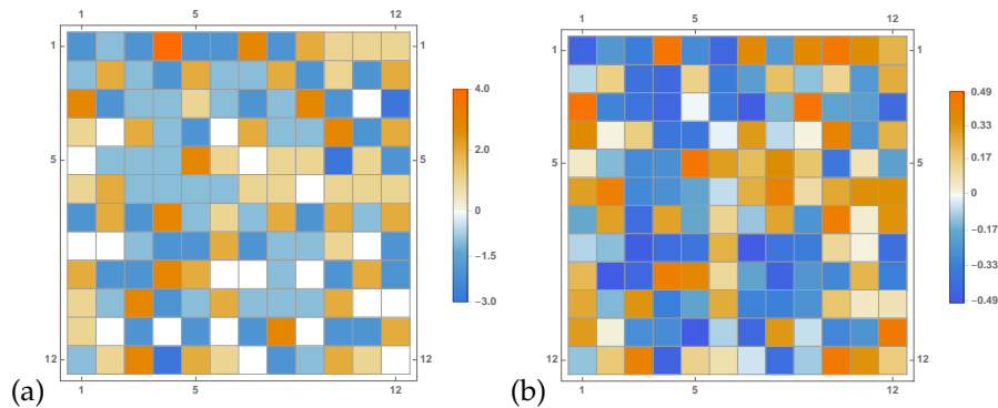
Figure 20.41: (a) An example of an admissible block M , initiated by a guess block with many m_z = 4 . Row 1, column 3 site is the only one with m_{(3,12)} = 4 . (b) The corresponding invariant 2-torus.
