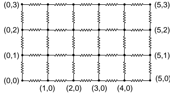
Figure 6.5: A [5 \times 4] rectangular resistor network: resistors with resistances r and s on edges of the network in, respectively, horizontal and vertical directions.
