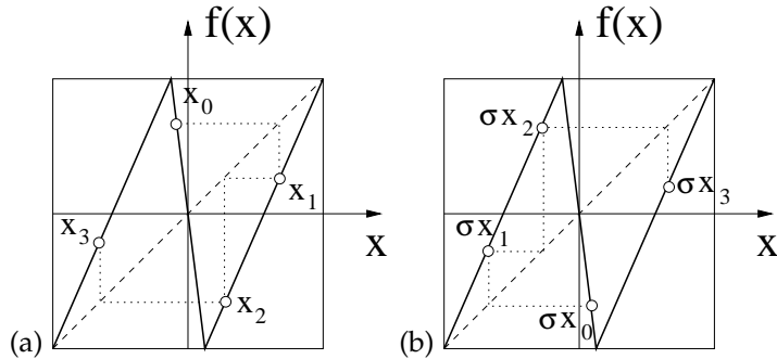
Figure 5.4: The bimodal Ulam sawtooth map with the D_1 symmetry f(-x) = -f(x) . If the trajectory (a) x_0 \rightarrow x_1 \rightarrow x_2 \rightarrow \dots is a solution, so is its reflection (b) \sigma x_0 \rightarrow \sigma x_1 \rightarrow \sigma x_2 \rightarrow \dots . (work through example 5.6; continued in figure 5.5).
