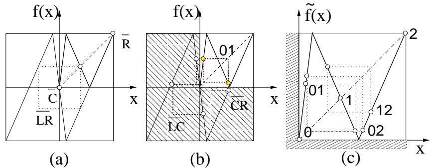
Figure 5.6: The bimodal Ulam sawtooth map of figure 5.5 with the D_1 symmetry f(-x) = -f(x) , restricted to the fundamental domain. f(x) is indicated by the thin line, and fundamental domain map \tilde{f}(\tilde{x}) by the thick line. (a) Boundary fixed point \bar{C} is the fixed point \bar{0} . The asymmetric fixed point pair \{\bar{L}, \bar{R}\} is reduced to the fixed point \bar{2} , and the full state space symmetric 2-cycle \bar{L}\bar{R} is reduced to the fixed point \bar{1} . (b) The asymmetric 2-cycle pair \{\bar{L}\bar{C}, \bar{C}\bar{R}\} is reduced to 2-cycle \bar{0}\bar{1} . (c) All fundamental domain fixed points and 2-cycles. (work through example 5.10) (Y. Lan,)
