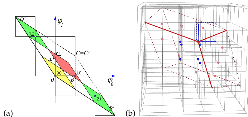
Figure 15.22: Was reffigfig:catCycJacob, now superannuated: (a) [2 \times 2] orbit Jacobian matrix \mathcal{J} refeqcatFundPar2 had a wrong sign, meaningless partition into 9 rectangles. (b) Han 2020-02-11: Intermediate attempt to draw reffigfig:catCycJacob. [3 \times 3] orbit Jacobian matrix \mathcal{J} had tons of irrelevant points plotted, is unintelligible.
