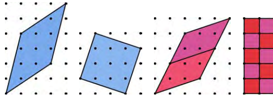
Figure 6.4: Four Bravais cells of area 10, a figure from Holmin’s PhD thesis [106]. The two blue Bravais cells are not ‘primitive’ (i.e., prime), as they are clearly tiled by smaller prime Bravais cells. Homlin claims that the two blue Bravais cells are primitive, but that is wrong, see (20.235).
