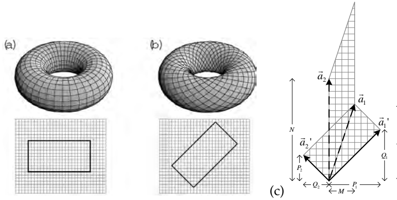
Figure 13.3: A helical tiling is formed by pairwise joining of the edges of the rectangle spanned by an orthogonal set of basis vectors in the \mathbb{Z}^2 lattice: (a) the direction of the basis vectors coincides with the lattice orientations for the conventional toroidal bc's, and (b) a helical torus. (c) Equivalence between the bc's in helical and twisted schemes prescribed by \{\vec{a}_1, \vec{a}_2\} and \{\vec{a}'_1, \vec{a}'_2\} respectively, on a [M \times N] square lattice. For the helical bc's, the setting Q_1/P_1 = Q_2/P_2 ensures that the two primitive vectors are orthogonal. On the other hand, twisting is generated by a d -unit traverse shift.
