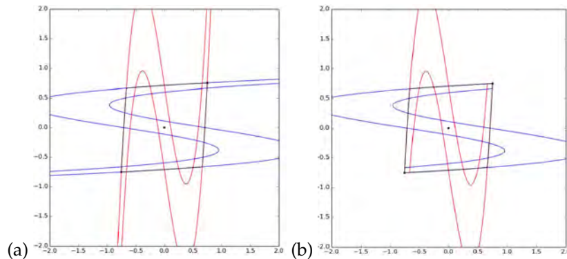
Figure 19.4: (Continued from figure 19.3.) (a) The intersections of fixed points' \phi_L, \phi_R stable-unstable manifolds form the level 0, single domain 'diamond' cover of the bimodal Smale horseshoe non-wandering set. (b) Iterating the 'diamond' forward and backward yield the level 2, 3^2 domains cover. As this is the Lo Fan [1] formulation of \phi^4 theory (19.6), g = 15, c = -8.5; \phi_L = -0.7527, \phi_R = 0.7527 , I will have to replot this for our group's formulation of \phi^4 theory. (Continued in figure 19.6).
