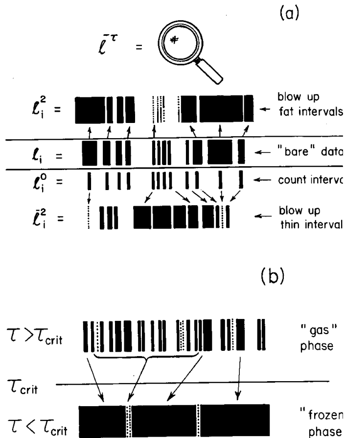
Figure A35.2: Different averages over a strange set.
