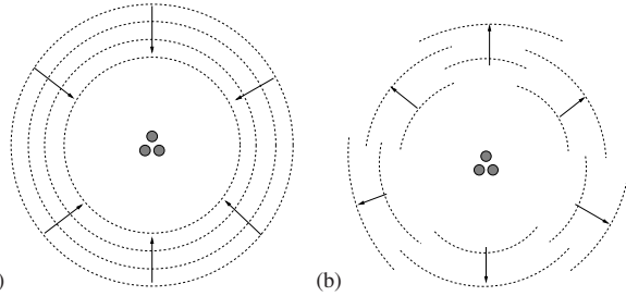
Figure 39.1: (a) Incoming spherical waves running into an obstacle. (b) Superposition of outgoing spherical waves scattered from an obstacle.
