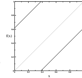
Figure 31.1: Unperturbed circle map ( k = 0 in (31.1)) with golden mean rotation number.
