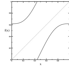
Figure 31.3: Critical circle map ( k = 1 in (31.1)) with golden mean bare rotation number.
