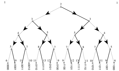
Figure 31.4: Farey tree: alternating binary ordered labeling of all Farey denominators on the n th Farey tree level.
