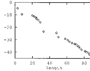
Figure 18.2: The logarithm \ln|z_0^{(n)} - z_0| of the difference between the leading zero of the n -th polynomial approximation to topological zeta function and our best estimate (18.23), as a function of order of the polynomial n (the topological zeta function evaluated for the closest value of A to A = 3.8 for which the quadratic map has a stable cycle of period n ). (from K.T. Hansen [9])
