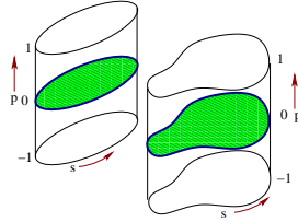
Figure 9.3: In D = 2 the billiard Poincaré section is a cylinder, with the parallel momentum p ranging over p \in [-1, 1] , and with the s coordinate is cyclic along each connected component of \partial Q . The rectangle figure 9.2(b) is such cylinder unfolded, with periodic boundary conditions glueing together the left and the right edge of the rectangle.
