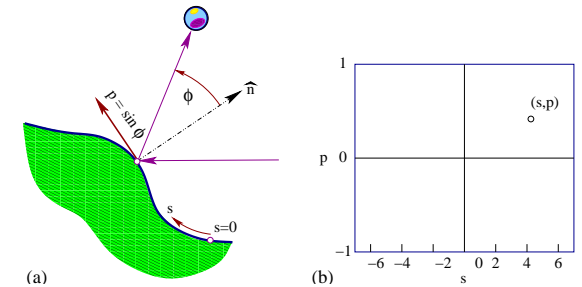
Figure 9.2: (a) A planar billiard trajectory is fixed by specifying the perimeter length parametrized by s and the outgoing trajectory angle \phi , both measured counterclockwise with respect to the outward normal \hat{n} . (b) The Birkhoff phase-space coordinate pair (s, p) fully specifies the trajectory, where p = |p| \sin \phi is the momentum component tangential to the boundary. As the pinball kinetic energy is conserved in elastic scattering, the pinball mass and the magnitude of the pinball momentum are customarily set to m = |p| = 1 .
