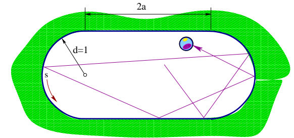
Figure 9.1: The stadium billiard [9.9, 9.10] is a 2-dimensional domain bounded by two semi-circles of radius d = 1 connected by two straight walls of length 2a . At the points where the straight walls meet the semi-circles, the curvature of the border changes discontinuously; these are the only singular points of the flow. The length a is the only parameter.
