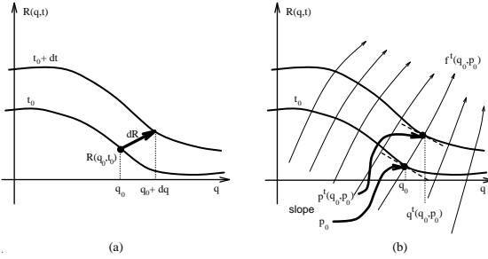
Figure 37.1: (a) A phase R(q,t) plotted as a function of the position q for two infinitesimally close times. (b) The phase R(q,t) transported by a swarm of “particles”; The Hamilton’s equations (37.10) construct R(q,t) by transporting q_0 \rightarrow q(t) and the slope of R(q_0, t_0) , that is p_0 \rightarrow p(t) .
