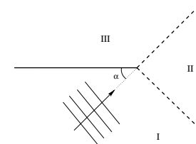
Figure 42.1: Scattering of a plane wave off a half line.
