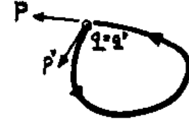
Figure 38.1: A returning trajectory in the configuration space. The orbit is periodic in the full phase space only if the initial and the final momenta of a returning trajectory coincide as well.
