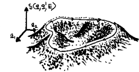
Figure 34.2: A romanticized sketch of S_p(E) = S(q, q, E) = \oint p(q, E) dq landscape orbit. Unstable periodic orbits traverse isolated ridges and saddles of the mountainous landscape of the action S(q_{||}, q_{\perp}, E) . Along a periodic orbit S_p(E) is constant; in the transverse directions it generically changes quadratically.
