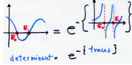
Figure 38.3: A sketch of how spectral determinants convert poles into zeros: The trace shows 1/(E - E_n) type singularities at the eigenenergies while the spectral determinant goes smoothly through zeroes.
