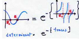
Figure 34.3: A sketch of how spectral determinants convert poles into zeros: The trace shows 1/(E - E_n) type singularities at the eigenenergies while the spectral determinant goes smoothly through zeroes.
