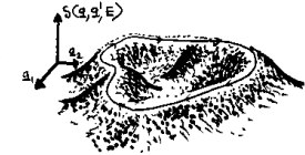
Figure 38.2: A romanticized sketch of S_\rho(E) = S(q, q, E) = \oint p(q, E) dq landscape orbit. Unstable periodic orbits traverse isolated ridges and saddles of the mountainous landscape of the action S(q_\parallel, q_\perp, E) . Along a periodic orbit S_\rho(E) is constant; in the transverse directions it generically changes quadratically.
