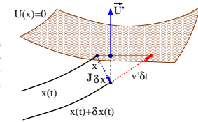
Figure 4.2: If x(t) intersects the Poincaré section \mathcal{P} at time \tau , the nearby x(t) + \delta x(t) trajectory intersects it time \tau + \delta \tau later. As (U' \cdot v' \delta \tau) = -(U' \cdot J \delta x) , the difference in arrival times is given by \delta \tau = -(U' \cdot J \delta x) / (U' \cdot v') .
