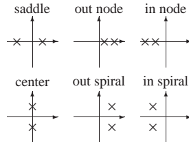
Figure 4.4: Qualitatively distinct types of exponents \{\lambda^{(1)}, \lambda^{(2)}\} of a [2 \times 2] Jacobian matrix.
