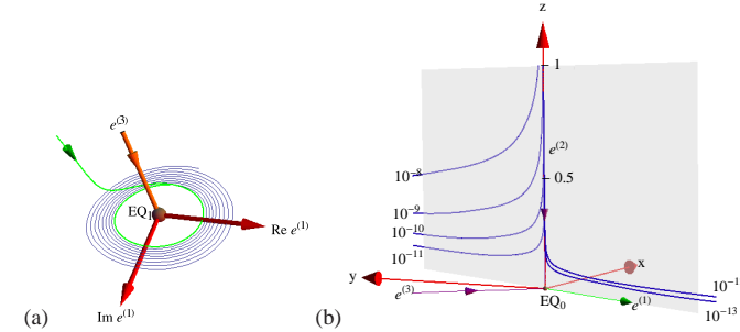
Figure 4.6: (a) A perspective view of the linearized Lorenz flow near E_{Q_1} equilibrium, see figure 3.4 (a). The unstable eigenplane of E_{Q_1} is spanned by \{\text{Re } e^{(1)}, \text{Im } e^{(1)}\} ; the stable subspace by the stable eigenvector e^{(3)} . (b) Lorenz flow near the E_{Q_0} equilibrium: unstable eigenvector e^{(1)} , stable eigenvectors e^{(2)}, e^{(3)} . Trajectories initiated at distances 10^{-8} \dots 10^{-12}, 10^{-13} away from the z -axis exit finite distance from E_{Q_0} along the (e^{(1)}, e^{(2)}) eigenvectors plane. Due to the strong \lambda^{(1)} expansion, the E_{Q_0} equilibrium is, for all practical purposes, unreachable, and the E_{Q_1} \rightarrow E_{Q_0} heteroclinic connection never observed in simulations such as figure 2.5. (E. Siminos; continued in figure 11.8.)
