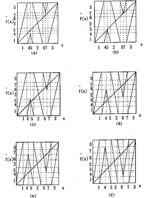
Figure O.1: (a)-(f) The sawtooth map (O.1) for the 6 values of parameter a for which the folding point of the map aligns with the endpoint of one of the 7 intervals and yields a finite Markov partition (from ref. [O.1]). The corresponding transition graphs are given in figure O.2.
