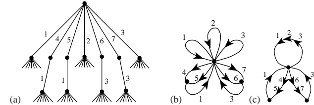
Figure O.2: (a) The sawtooth map (O.1) partition tree for figure O.1 (a); while intervals M_1, M_2, M_3 map onto the whole unit interval, f(M_1) = f(M_2) = f(M_3) = M_1 , intervals M_4, M_5 map onto M_1 only, f(M_4) = f(M_5) = M_1 , and similarly for intervals M_6, M_7 . An initial point starting out in the interval M_1, M_2 or M_3 can land anywhere on the unit interval, so the subtrees originating from the corresponding nodes on the partition tree are similar to the whole tree and can be identified (as, for example, in figure 14.5), yielding (b) the transition graph for the Markov partition of figure O.1 (a). (c) the transition graph in the compact notation of (25.26).
