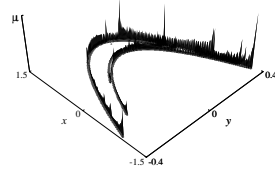
Figure 16.5: Natural measure (16.19) for the Hénon map (3.17) strange attractor at parameter values (a, b) = (1.4, 0.3) . See figure 3.6 for a sketch of the attractor without the natural measure binning. (Courtesy of J.-P. Eckmann)
