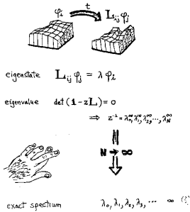
Figure 16.4: State space discretization approach to computing averages.
