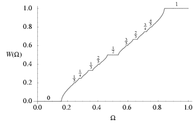
Figure 31.2: The critical circle map ( k = 1 in (31.1)) devil's staircase [31.2]; the winding number W as function of the parameter \Omega .
