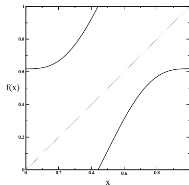
Figure 27.3: Critical circle map ( k = 1 in (27.1)) with golden mean bare rotation number.
