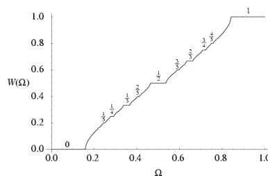
Figure 27.2: The critical circle map ( k = 1 in (27.1)) devil's staircase [27.3]; the winding number W as function of the parameter \Omega .
