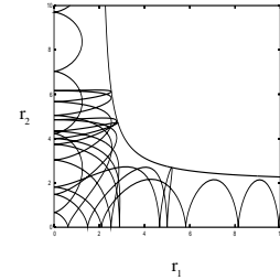
Figure 34.1: A typical collinear helium trajectory in the r_1 - r_2 plane; the trajectory enters along the r_1 axis and escapes to infinity along the r_2 axis.
