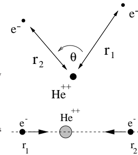
Figure 37.1: Coordinates for the helium three body problem in the plane.
