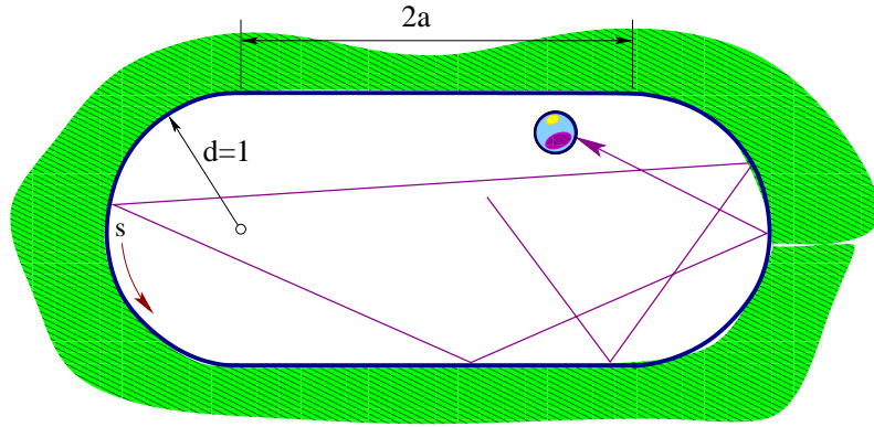
Figure 8.1: The stadium billiard [8.9, 8.10] is a 2-dimensional domain bounded by two semi-circles of radius d = 1 connected by two straight walls of length 2a . At the points where the straight walls meet the semi-circles, the curvature of the border changes discontinuously; these are the only singular points of the flow. The length a is the only parameter.
