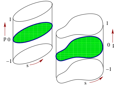
Figure 8.3: In D = 2 the billiard Poincaré section is a cylinder, with the parallel momentum p ranging over p \in \{-1, 1\} , and with the s coordinate is cyclic along each connected component of \partial Q . The rectangle figure 8.2(b) is such cylinder unfolded, with periodic boundary conditions glueing together the left and the right edge of the rectangle.
