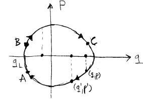
Figure 32.2: A 1-dof phase space trajectory of a particle moving in a bound potential.
