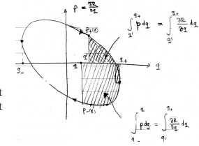
Figure 32.3: S_p(E) , the action of a periodic orbit p at energy E , equals the area in the phase space traced out by the 1-dof trajectory.
