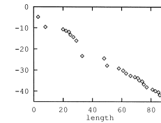
Figure 15.2: The logarithm \ln|z_0^{(n)} - z_0| of the difference between the leading zero of the n -th polynomial approximation to topological zeta function and our best estimate (15.33), as a function of order of the polynomial n (the topological zeta function evaluated for the closest value of A to A = 3.8 for which the quadratic map has a stable cycle of period n ). (from K.T. Hansen [12.22])
