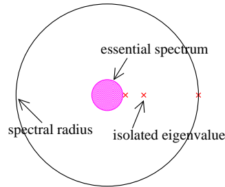
Figure 23.5: Spectrum of the Perron-Frobenius operator acting on the space of \mathbb{C}^{k+\alpha} Hölder-continuous functions: only k isolated eigenvalues remain between the spectral radius, and the essential spectral radius which bounds the “essential,” continuous spectrum.
