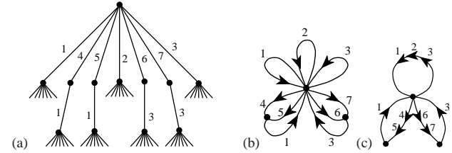
Figure T.2: (a) The sawtooth map (T.1) partition tree for figure T.1 (a); while intervals \mathcal{M}_1, \mathcal{M}_2, \mathcal{M}_3 map onto the whole unit interval, f(\mathcal{M}_1) = f(\mathcal{M}_2) = f(\mathcal{M}_3) = \mathcal{M}_1 , intervals \mathcal{M}_4, \mathcal{M}_5 map onto \mathcal{M}_1 only, f(\mathcal{M}_4) = f(\mathcal{M}_5) = \mathcal{M}_1 , and similarly for intervals \mathcal{M}_6, \mathcal{M}_7 . An initial point starting out in the interval \mathcal{M}_1, \mathcal{M}_2 or \mathcal{M}_3 can land anywhere on the unit interval, so the subtrees originating from the corresponding nodes on the partition three are similar to the whole tree and can be identified (as, for example, in figure 14.5), yielding (b) the transition graph for the Markov partition of figure T.1 (a). (c) the transition graph in the compact notation of (25.26).
