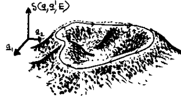
Figure 33.2: A romanticized sketch of S_p(E) = S(q, q, E) = \oint p(q, E) dq landscape orbit. Unstable periodic orbits traverse isolated ridges and saddles of the mountainous landscape of the action S(q_{\parallel}, q_{\perp}, E) . Along a periodic orbit S_p(E) is constant; in the transverse directions it generically changes quadratically.
