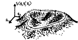
Figure 33.2: A romanticized sketch of S_p(E) = S(q, q, E) = \oint p(q, E) dq landscape orbit. Unstable periodic orbits traverse isolated ridges and saddles of the mountainous landscape of the action S(q_{||}, q_{\perp}, E) . Along a periodic orbit S_p(E) is constant; in the transverse directions it generically changes quadratically.
