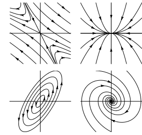
Figure 4.4: Streamlines for several typical 2-dimensional flows: saddle (hyperbolic), in node (attracting), center (elliptic), in spiral.
