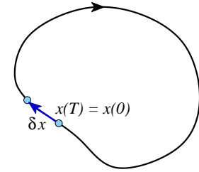
Figure 4.3: For a periodic orbit p , any two points along the cycle are mapped into themselves after one cycle period T , hence \delta x = v(x_0)\delta t is mapped into itself by the cycle fundamental matrix J_p .
