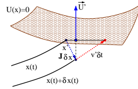
Figure 4.8: If x(t) intersects the Poincaré section \mathcal{P} at time \tau , the nearby x(t) + \delta x(t) trajectory intersects it time \tau + \delta\tau later. As (U' \cdot v \delta\tau) = -(U' \cdot J \delta x) , the difference in arrival times is given by \delta\tau = -(U' \cdot J \delta x)/(U' \cdot v) .
