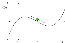
Figure 27.1: “Potential” V_i(x) (27.7) for a typical point along an initial guess trajectory. For \sigma_i = +1 the flow is toward the local maximum of V_i(x) , and for \sigma_i = -1 toward the local minimum. A large deviation of x_i 's is needed to destabilize a trajectory passing through such local extremum of V_i(x) , hence the basin of attraction is expected to be large.
