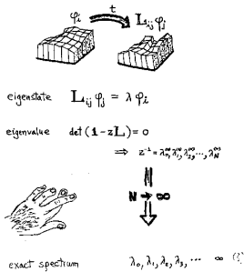
Figure 14.4: State space discretization approach to computing averages.
