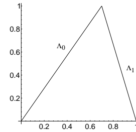
Figure 14.3: A piecewise-linear skew “Ulam tent” map (14.11) ( \Lambda_0 = 4/3, \Lambda_1 = -4 ).
