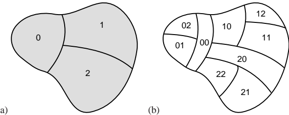
Figure 14.1: (a) First level of partitioning: A coarse partition of \mathcal{M} into regions \mathcal{M}_0 , \mathcal{M}_1 , and \mathcal{M}_2 . (b) n = 2 level of partitioning: A refinement of the above partition, with each region \mathcal{M}_i subdivided into \mathcal{M}_{i0} , \mathcal{M}_{i1} , and \mathcal{M}_{i2} .
