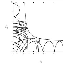
Figure 29.1: A typical collinear helium trajectory in the r_1 - r_2 plane; the trajectory enters along the r_1 axis and escapes to infinity along the r_2 axis.
