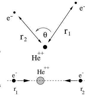
Figure 36.1: Coordinates for the helium three body problem in the plane.
