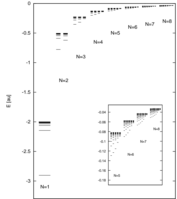
Figure 36.6: The exact quantum helium spectrum for L = 0 . The energy levels denoted by bars have been obtained from full 3-dimensional quantum calculations [3].
