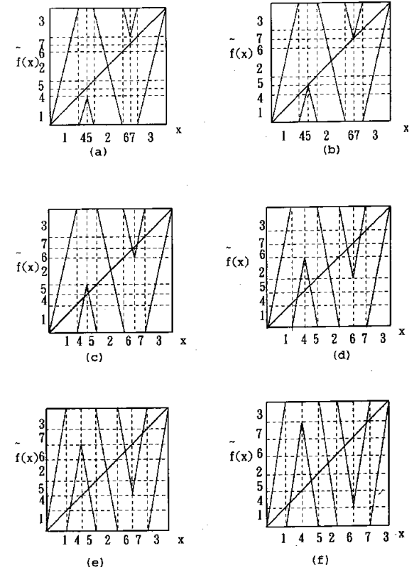
Figure A46.1: (a)-(f) The sawtooth map (A46.1) for the 6 values of parameter a for which the folding point of the map aligns with the endpoint of one of the 7 intervals and yields a finite Markov partition (from ref. [A46.1]). The corresponding transition graphs are given in figure A46.2.
