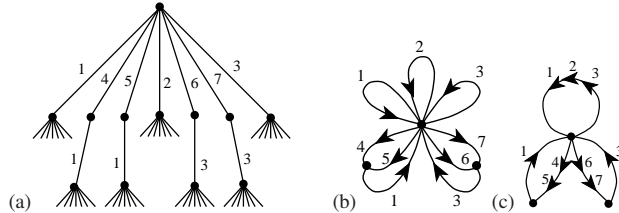
Figure A46.2: (a) The sawtooth map (A46.1) partition tree for figure A46.1 (a); while intervals M_1, M_2, M_3 map onto the whole unit interval, f(M_1) = f(M_2) = f(M_3) = M_1 , intervals M_4, M_5 map onto M_1 only, f(M_4) = f(M_5) = M_1 , and similarly for intervals M_6, M_7 . An initial point starting out in the interval M_1, M_2 or M_3 can land anywhere on the unit interval, so the subtrees originating from the corresponding nodes on the partition tree are similar to the whole tree and can be identified (as, for example, in figure 17.6), yielding (b) the transition graph for the Markov partition of figure A46.1 (a). (c) the transition graph in the compact notation of (24.26).
