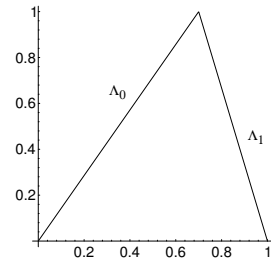
Figure 19.3: The piecewise-linear skew ‘full tent map’ (19.37), with \Lambda_0 = 4/3 , \Lambda_1 = -4 . See example 19.1.
