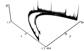
Figure 19.5: Natural measure (19.16) for the Hénon map (3.17) strange attractor at parameter values (a, b) = (1.4, 0.3) . See figure 3.6 for a sketch of the attractor without the natural measure binning. See example 19.2. (Courtesy of J.-P. Eckmann)
