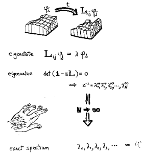
Figure 19.4: State space discretization approach to computing averages.
