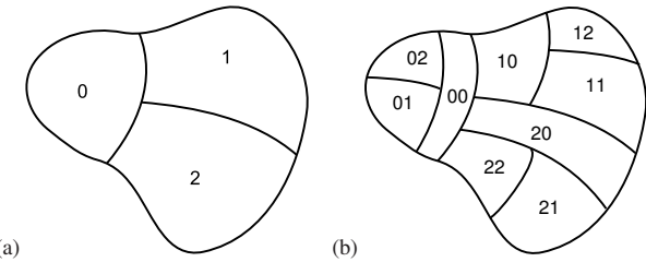
Figure 19.1: (a) First level of partitioning: A coarse partition of M into regions M_0 , M_1 , and M_2 . (b) n = 2 level of partitioning: A refinement of the above partition, with each region M_i subdivided into M_{i0} , M_{i1} , and M_{i2} .
