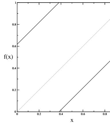
Figure 32.1: Unperturbed circle map ( k = 0 in (32.1)) with golden mean rotation number.
