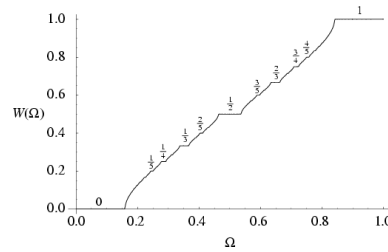
Figure 32.2: The critical circle map ( k = 1 in (32.1)) devil's staircase [18]; the winding number W as function of the parameter \Omega .
