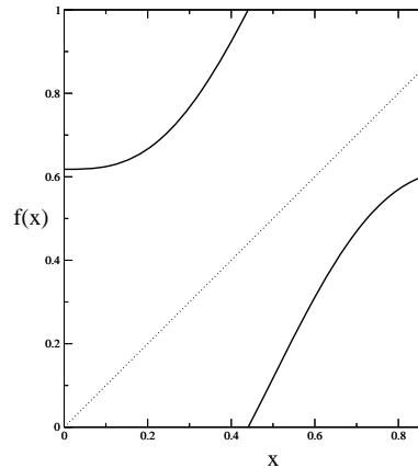
Figure 32.3: Critical circle map ( k = 1 in (32.1)) with golden mean bare rotation number.
