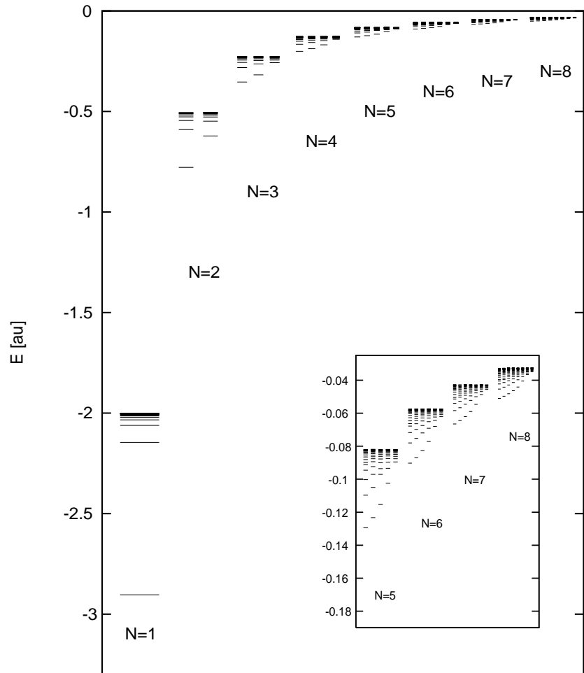
Figure 41.6: The exact quantum helium spectrum for L = 0 . The energy levels denoted by bars have been obtained from full 3-dimensional quantum calculations [41.3].
