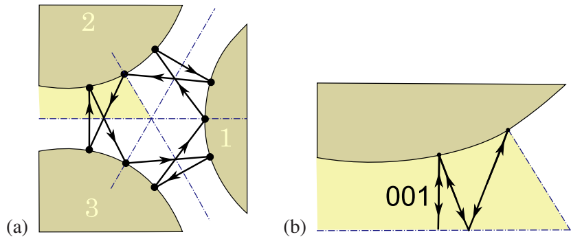
Figure 11.6: (a) The pair of full-space 9-cycles, the counter-clockwise 121232313 and the clockwise 131323212 correspond to (b) one fundamental domain 3-cycle 00\bar{1} .
