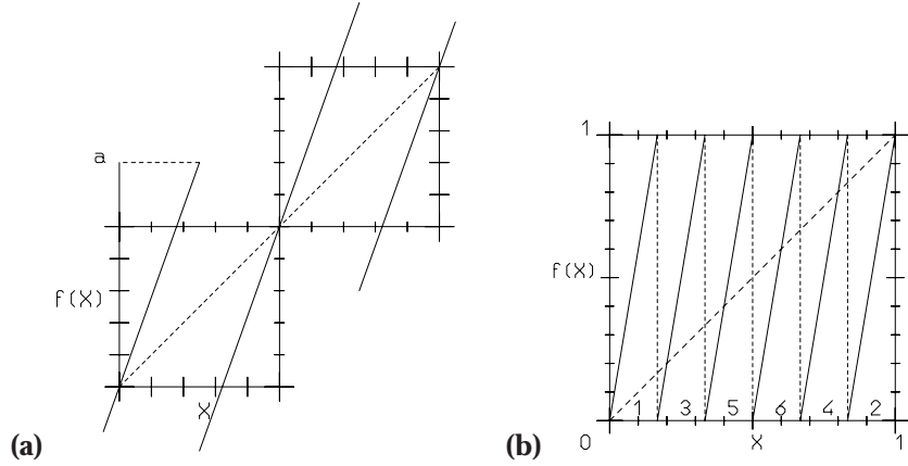
Fig. 23.3 (a) \hat{f}(\hat{x}) , the full space sawtooth map (23.9), \Lambda > 2 . (b) f(x) , the sawtooth map restricted to the unit circle (23.12), \Lambda = 6 .
