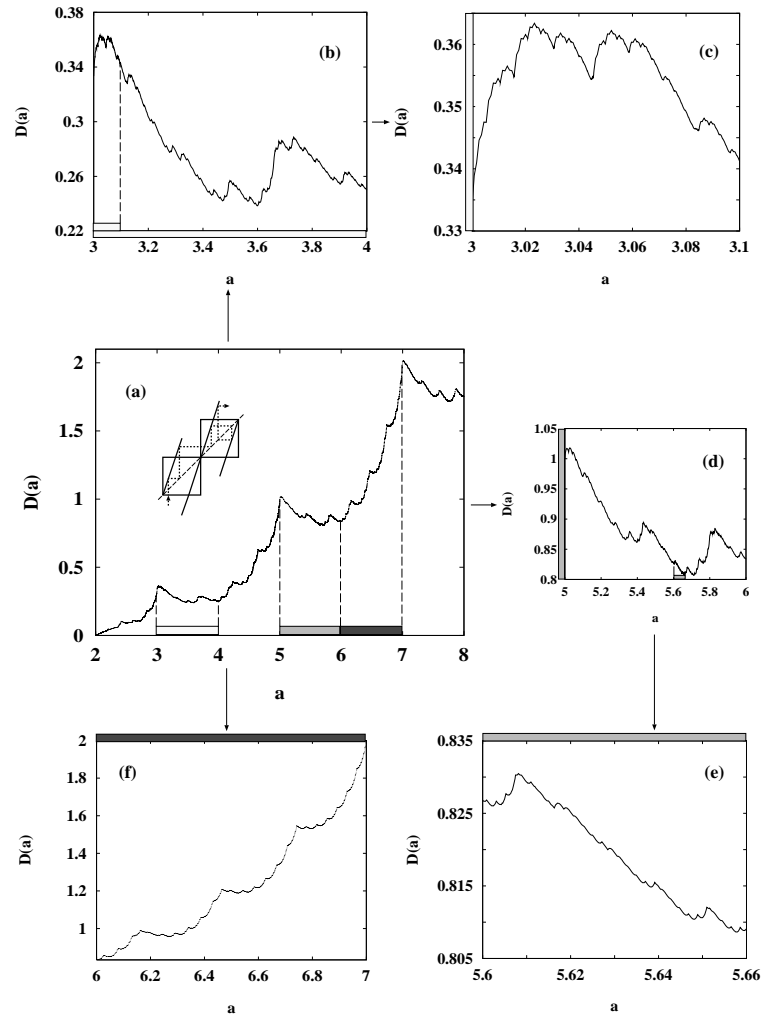
Fig. 23.5 The dependence of D on the map parameter a is continuous, but not monotone. (From Ref. [7]). Here a stands for the slope \Lambda in (23.9).
