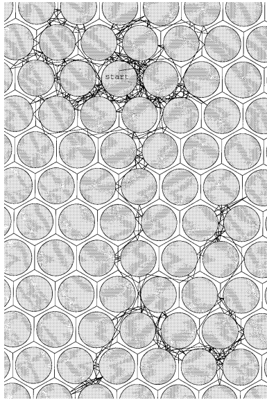
Fig. 23.1 Deterministic diffusion in a finite horizon periodic Lorentz gas. (Courtesy of T. Schreiber)
