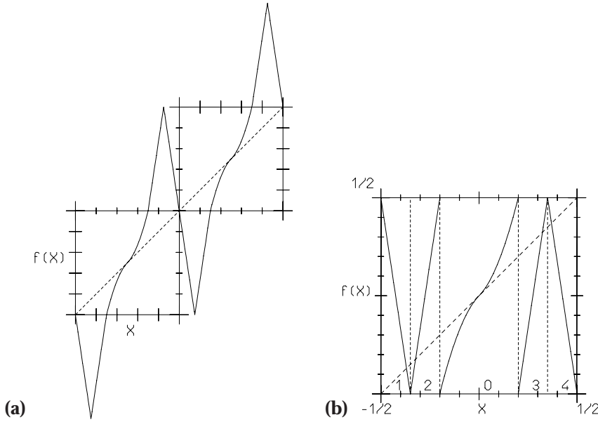
Fig. 23.6 (a) A map with marginal fixed point. (b) The map restricted to the unit circle.
