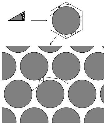
Fig. 23.2 Tiling of \hat{\mathcal{M}} , a periodic lattice of reflecting disks, by the fundamental domain \tilde{\mathcal{M}} . Indicated is an example of a global trajectory \hat{x}(t) together with the corresponding elementary cell trajectory x(t) and the fundamental domain trajectory \tilde{x}(t) . (Courtesy of J.-P. Eckmann)
