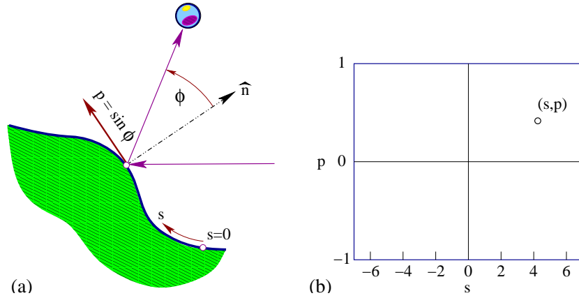
Fig. 8.2 (a) A planar billiard trajectory is fixed by specifying the perimeter length parametrized by s and the outgoing trajectory angle \phi , both measured counter-clockwise with respect to the outward normal \hat{n} . (b) The Birkhoff phase space coordinate pair (s, p) fully specifies the trajectory, where p = |p| \sin \phi is the momentum component tangential to the boundary (and we set |p| = 1 whenever convenient).
