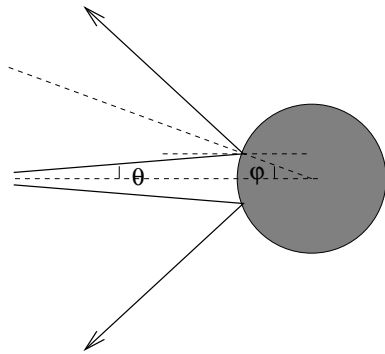
Fig. 8.4 Defocusing of a beam of nearby trajectories at a billiard collision. (A. Wirzba)
