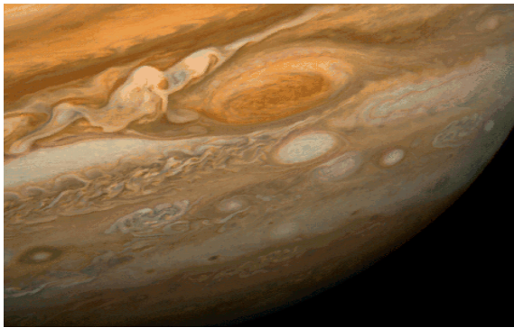
FIG. 3 The Great Red Spot, an anti-cyclonic vortex in the upper atmosphere of Jupiter. It has existed at least since it was observed in 1610 by Galileo Galilei with one of the first telescopes and measures 14,000 km north-south and 40,000 km east-west. Similar large-scale, long-lived vortices exist in the atmospheres of the other gas giant planets of our solar system. Features of “small-scale” turbulence can be clearly seen in the picture.
