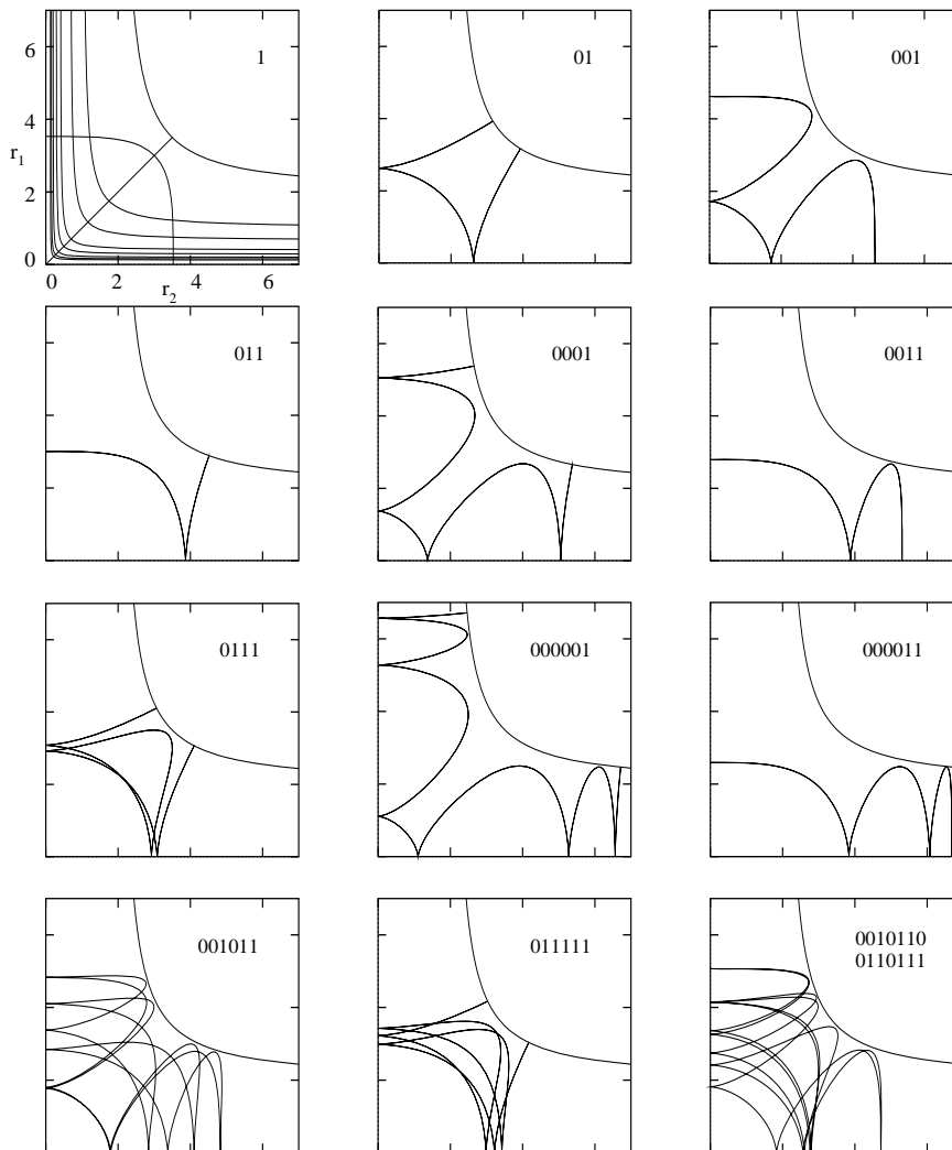
Figure 42.5: Some of the shortest cycles in collinear helium. The classical collinear electron motion is bounded by the potential barrier -1 = -2/r_1 - 2/r_2 + 1/(r_1 + r_2) and the condition r_i \geq 0 . The orbits are shown in the full r_1 - r_2 domain, the itineraries refers to the dynamics in the r_1 \geq r_2 fundamental domain. The last figure, the 14-cycle 00101100110111, is an example of a typical cycle with no symmetry.
